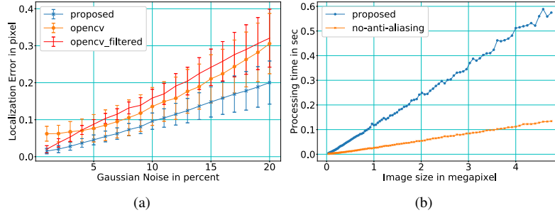
Figure 7: (a) Localization error over Gaussian noise of a modified baseline method using an additional filter stage of \sigma = 3 ; (b) processing time for corner detection and localization with and without anti-aliasing.
