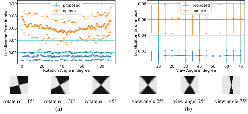
Figure 6: Localization error of the proposed method for a checkerboard corner: (a) localization error over rotation angle; (b) localization error over viewing angle
